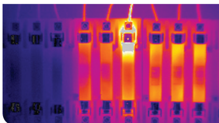
Overloaded fuse
